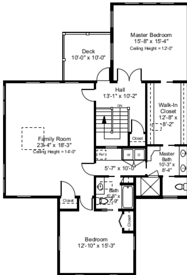
Second Floor Plan Ceiling Height = 8'-3"
