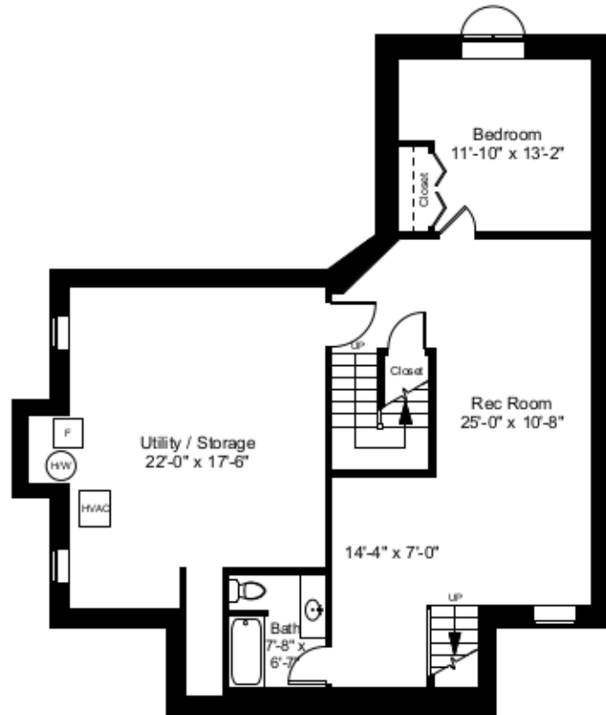
Lower Level Plan Ceiling Height = 7'-2"
